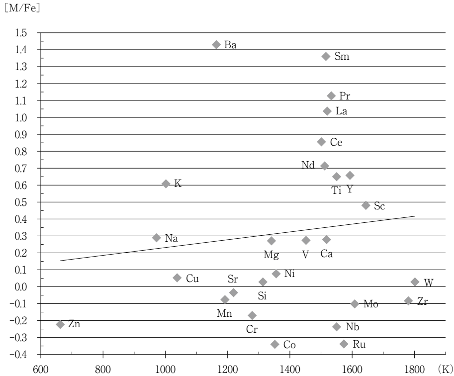
Fig. 3 The correlation between the relative abundance, [M/Fe]_{\text{HD37124}} - [M/Fe]_{\epsilon\text{Eri}} , and the 50% condensation temperature. The solid line shows the least-squares solution
