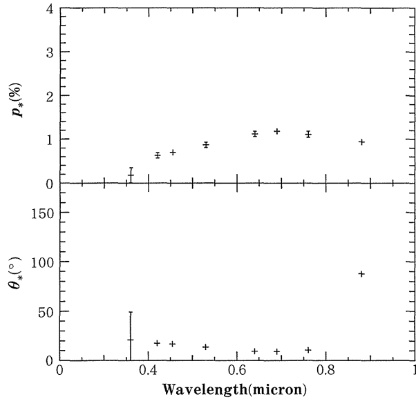
Fig.8. Wavelength dependence of the p_* and \theta_* values of U Mon. on 1998 February 10/11. The p_* values show a marginal \lambda^{-1} type dependence.
