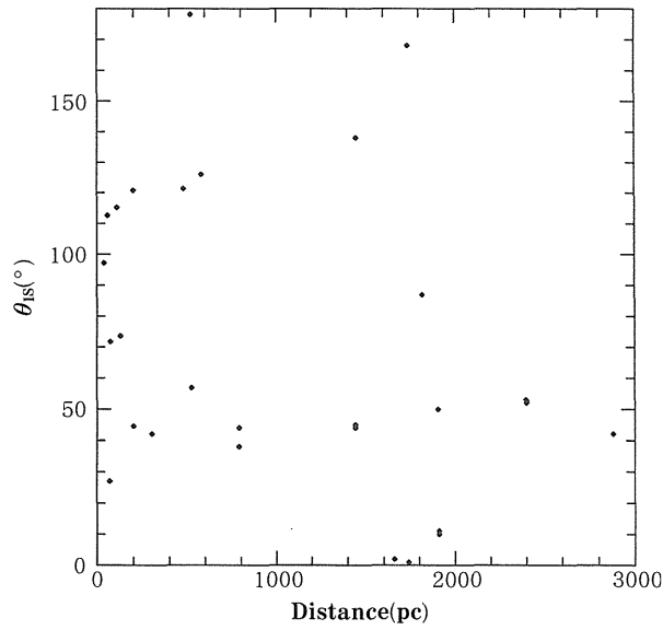
Fig.9. Dependence of the \theta_{1s} values near R Sct on distance. All the data are plotted.
