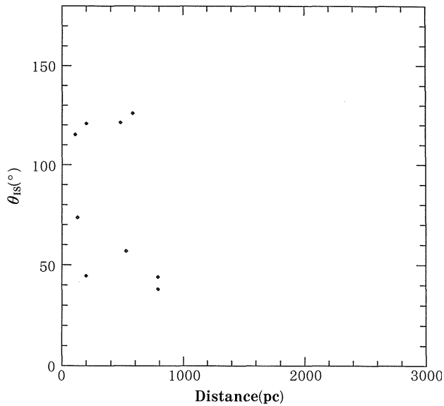
Fig.10. Dependence of the \theta_{1s} values near R Sct on distance. The data are plotted which satisfy the following conditions; d \leq 1000 pc, 18^{\text{h}}33^{\text{m}} \leq \alpha_{1950} \leq 19^{\text{h}} , and \delta_{1950} \geq -10^{\circ} .
