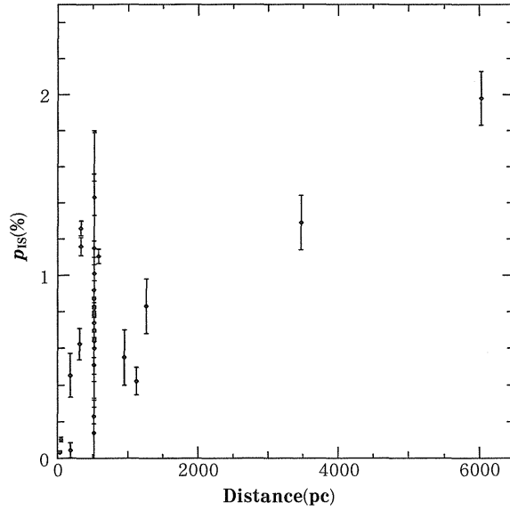
Fig.7. Dependence of the p_{is}(V) values near U Mon on distance. The scatter of the p_{is}(V) values is large for the stars within 2000pc.
